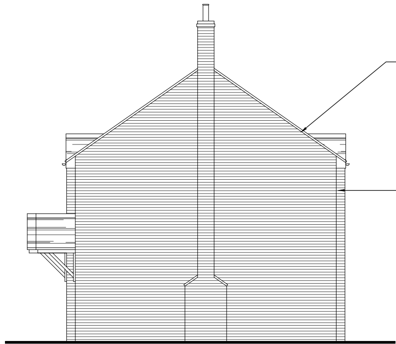
SIDE ELEVATION (1:100)
