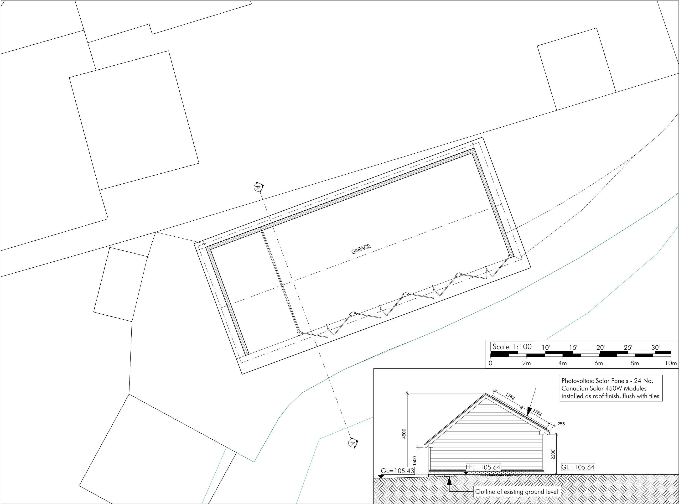
Proposed site layout plan
