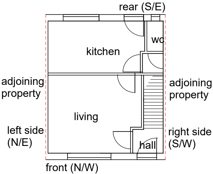
GROUND FLOOR LAYOUT
