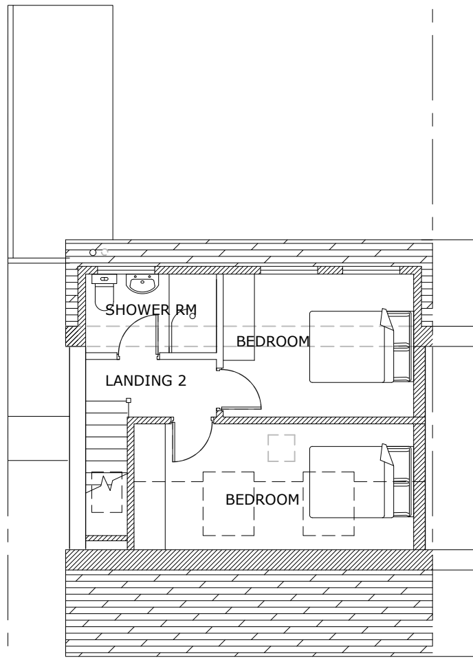
LOFT FLOOR
