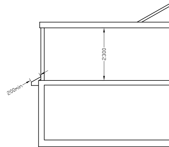
PROPOSED SECTION
