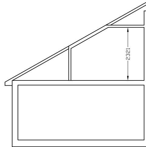
EXISTING SECTION
