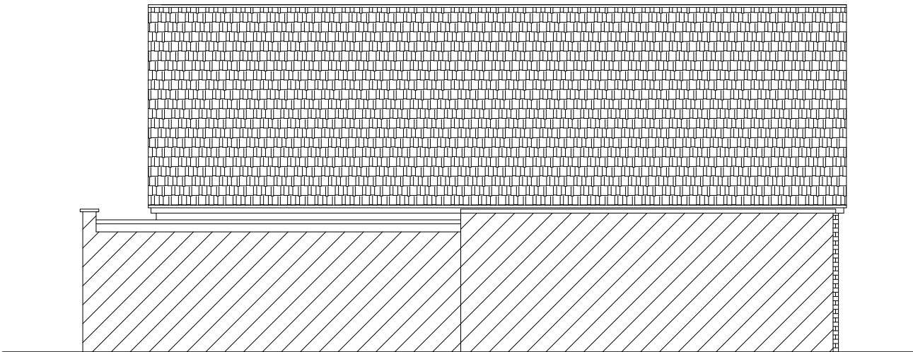
02 A-304 EXISTING RIGHT ELEVATION SCALE- 1:100@A3
