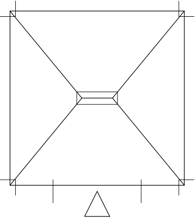
Roof Plan
