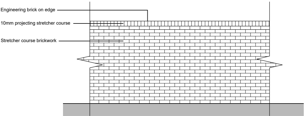
1800mm Brick Screen Wall
