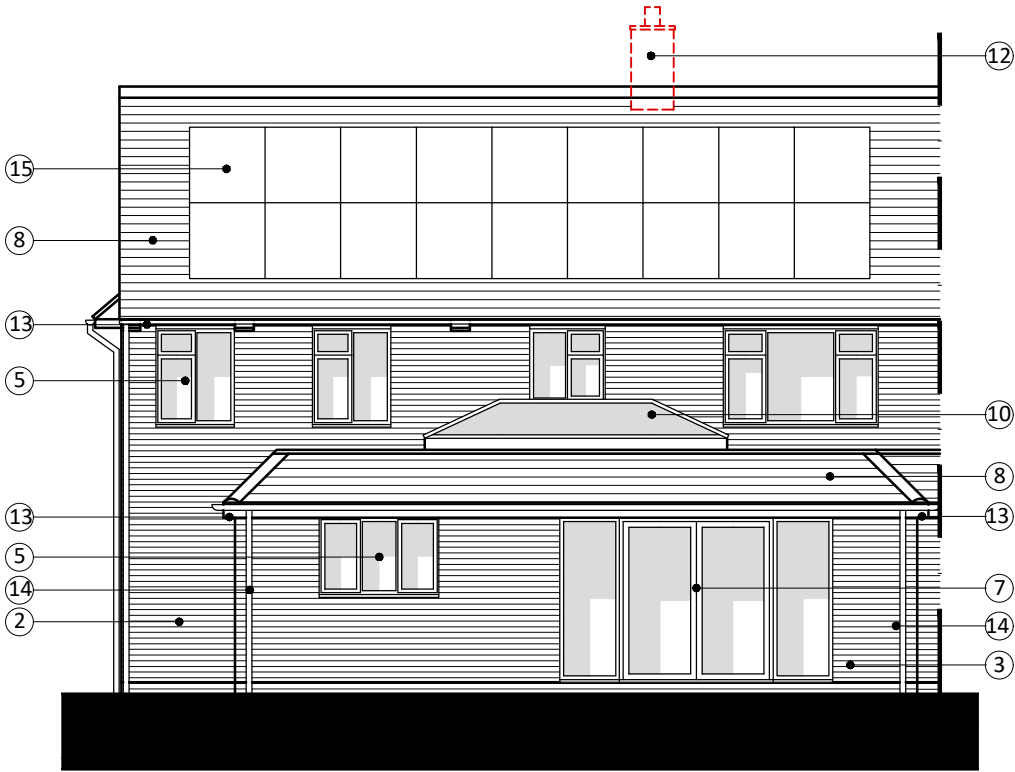
REAR ELEVATION (C-C)
