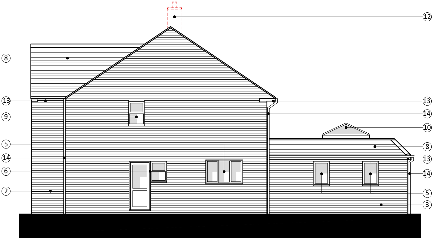
SIDE ELEVATION (D-D)
