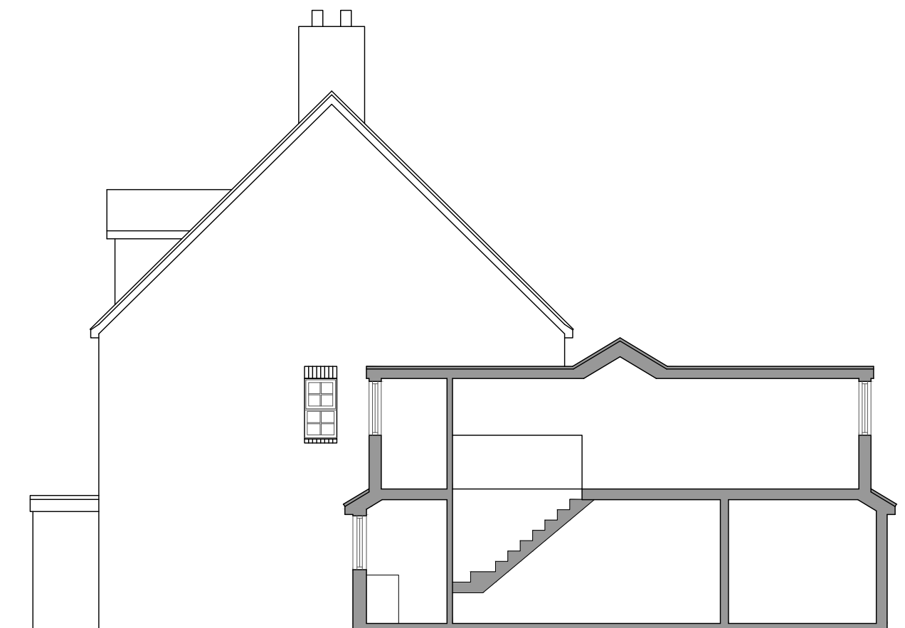
Section
