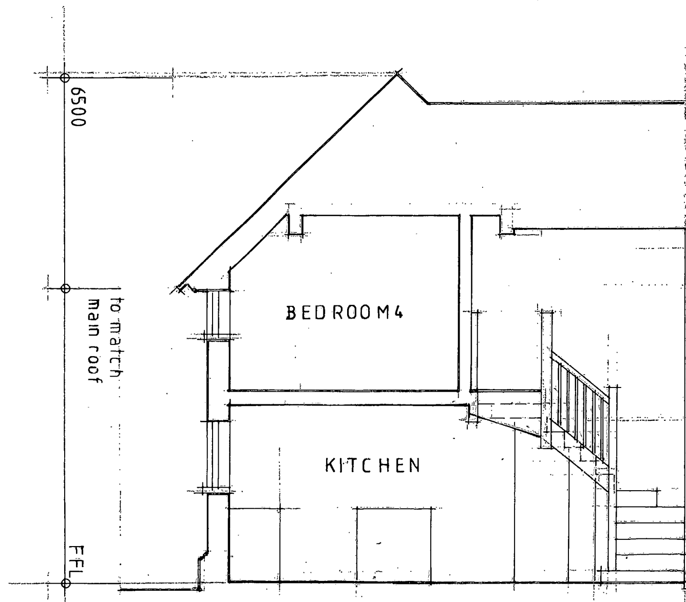
SECTION THRO' EXTENSION
