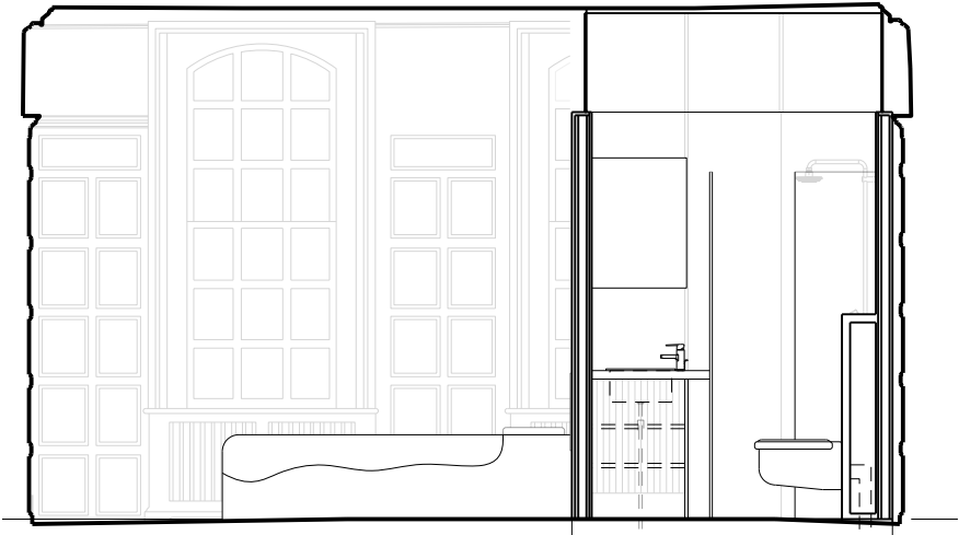
C Boudoir Bathroom Pod ~ Section A - A
