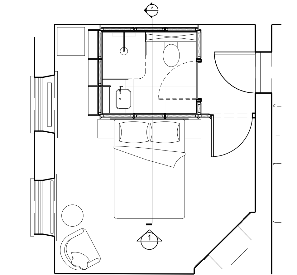
A Boudoir Bathroom Pod ~ Plan
