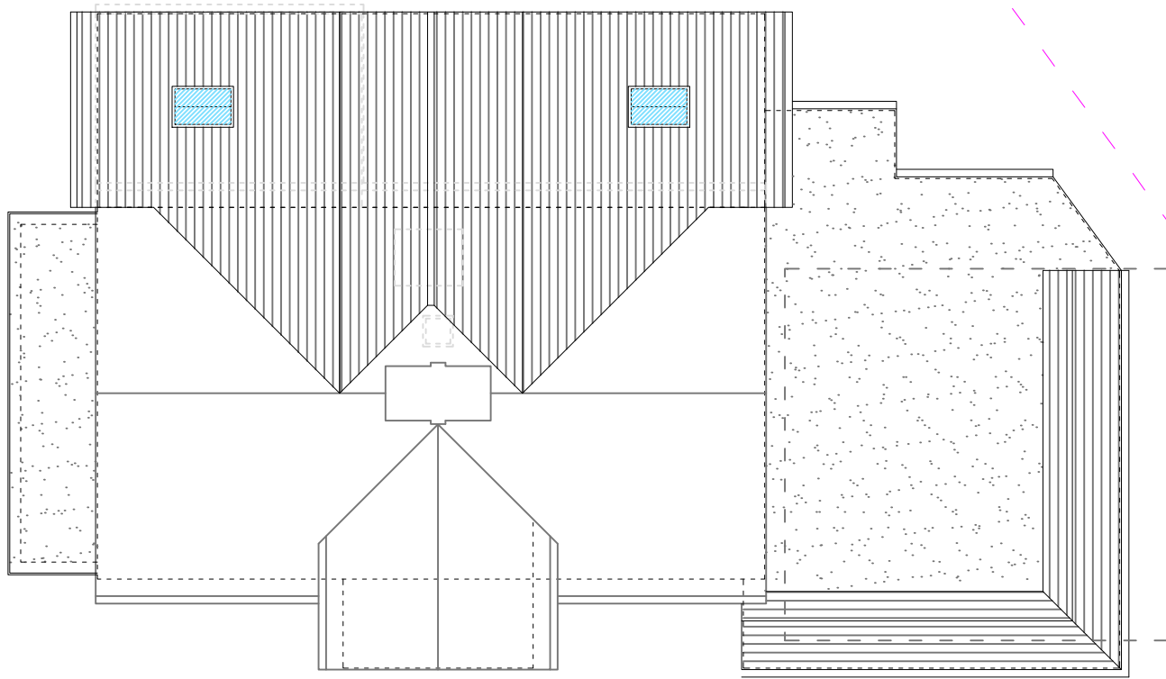
ROOF PLAN
