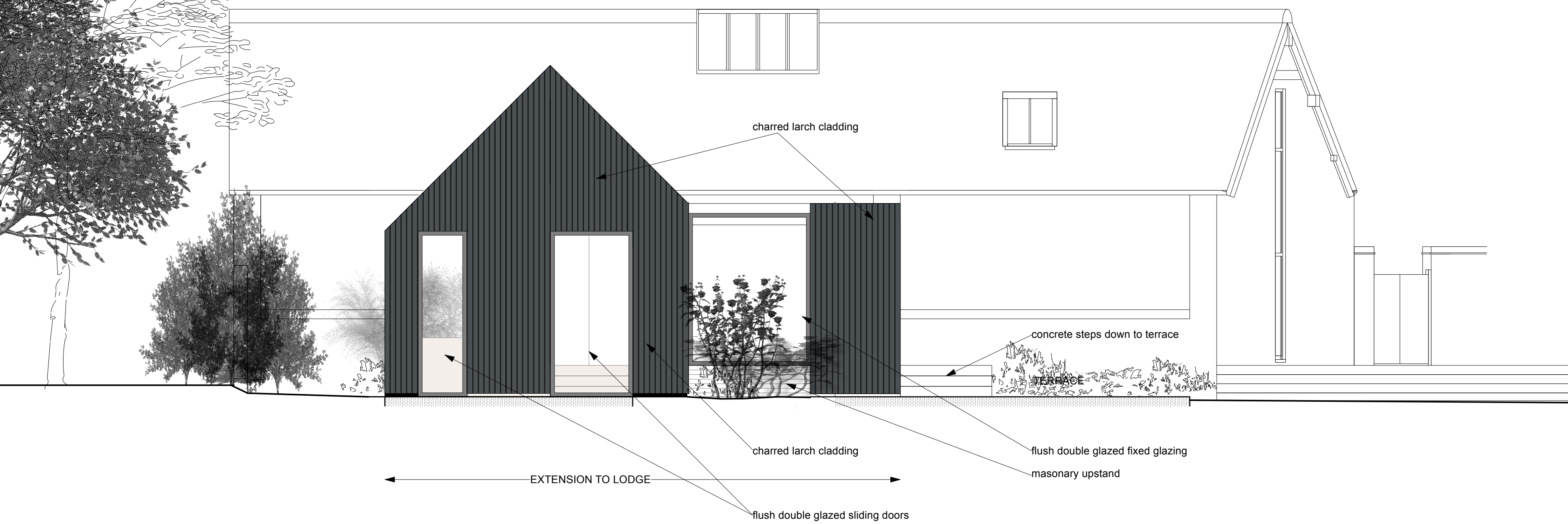
NORTH ELEVATION AS PROPOSED
