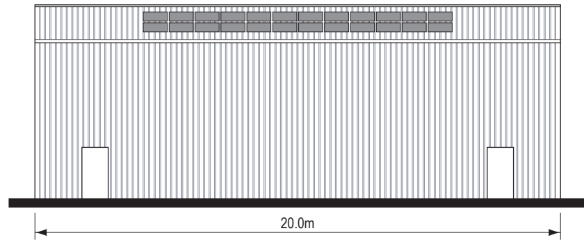
West Elevation
