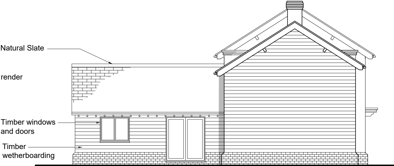
South Elevation
