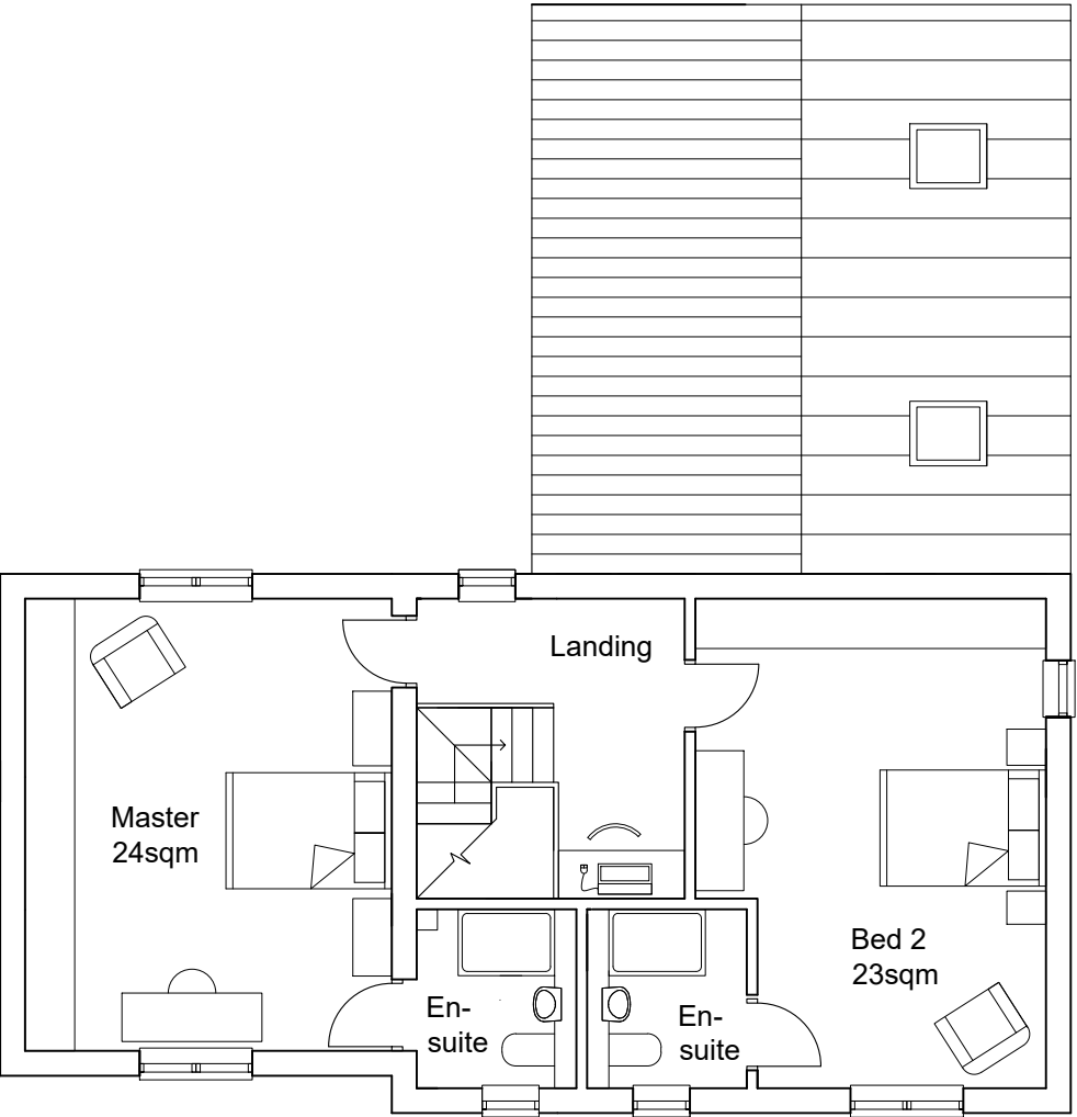
First Floor
