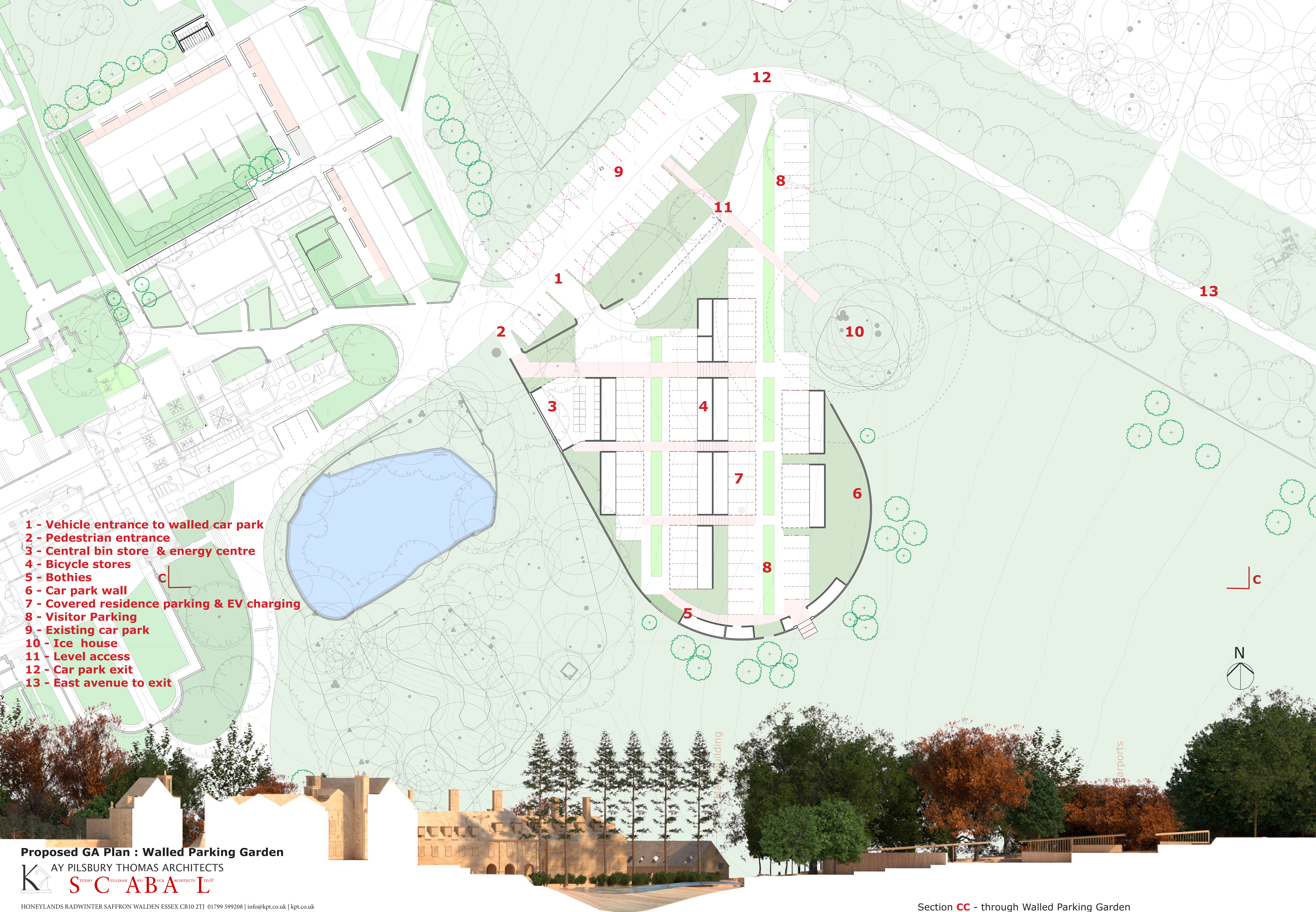
Section CC - through Walled Parking Garden
