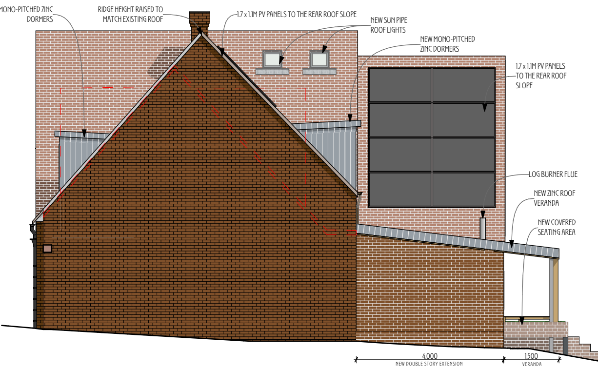
E-04 West Elevation 1:100
