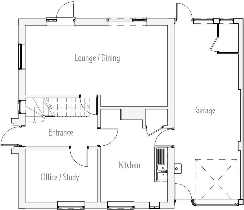
GF Ground Floor Plan 1:100
