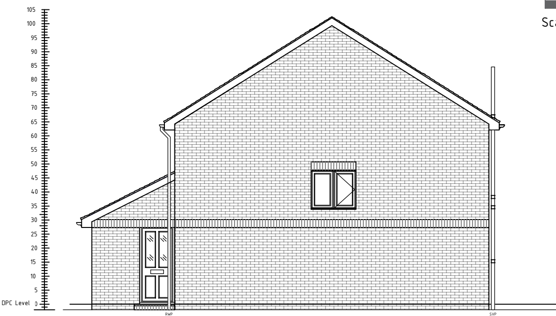
Existing Side Elevation 'A' @ 1:100
