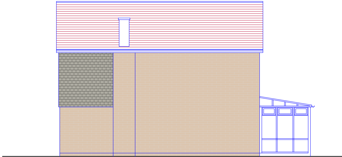
⊕ SIDE ELEVATION (WEST) AS EXISTING
