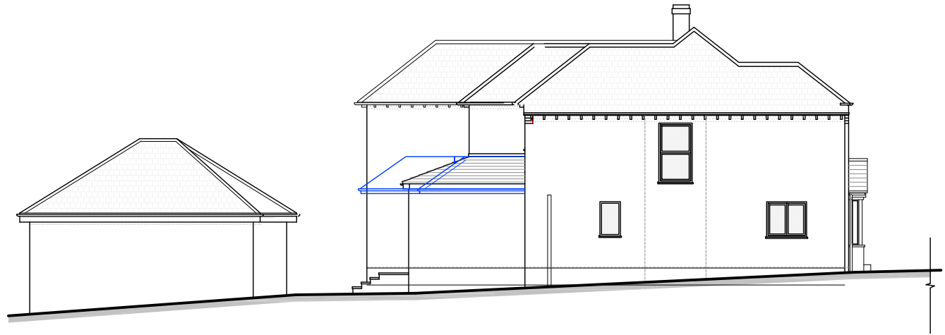
2205 sk 3 amended proposal elevations with the outline of the approved scheme overlaid
