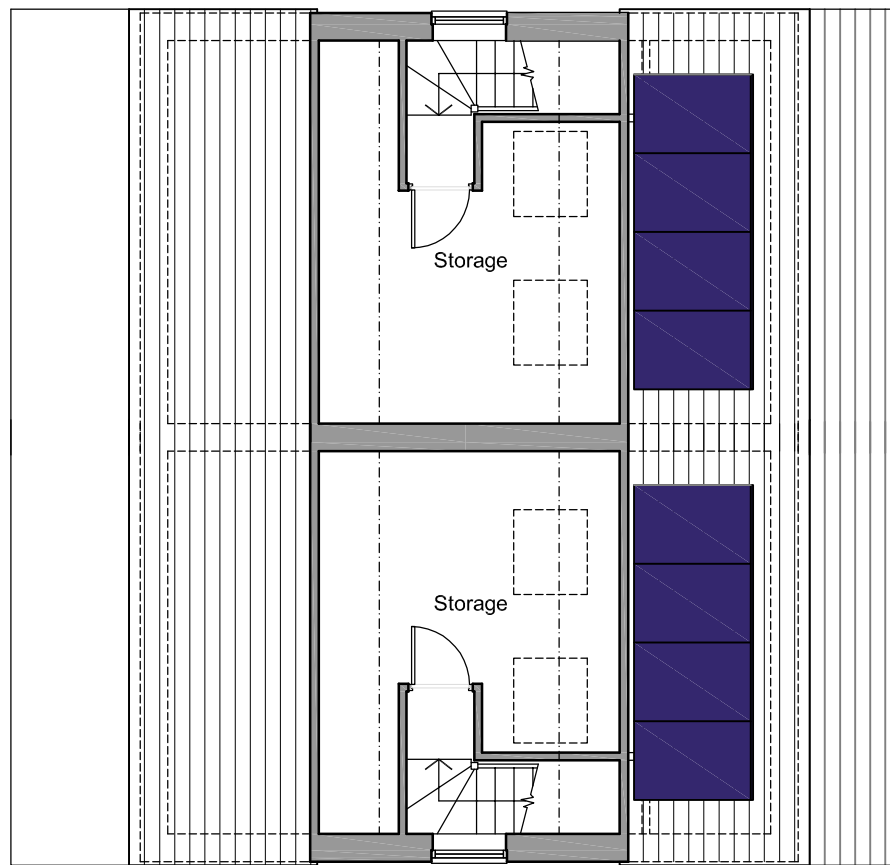
PROPOSED SECOND FLOOR PLAN (16m²) HOUSES 2 & 3
