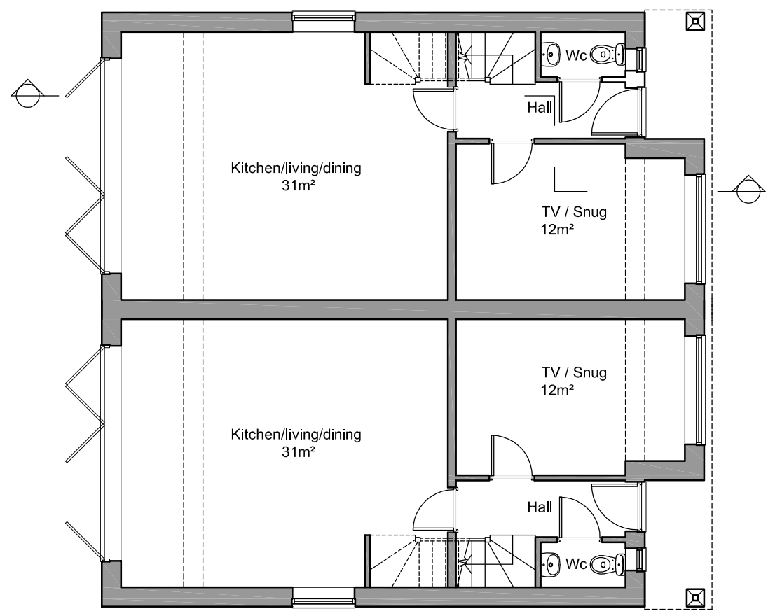
PROPOSED GROUND FLOOR PLAN (51.2m²) HOUSES 2 & 3
