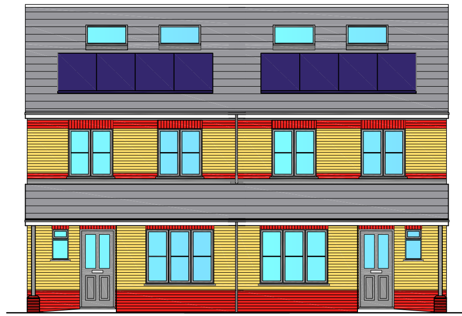
PROPOSED EAST FRONT ELEVATION HOUSE 2 & 3
