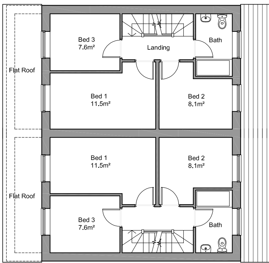
PROPOSED FIRST FLOOR PLAN (40.3m²) HOUSES 2 & 3
