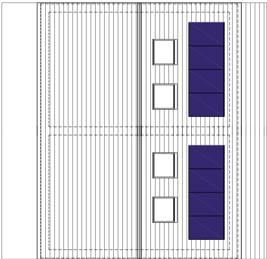
PROPOSED ROOF PLAN HOUSES 2 & 3
