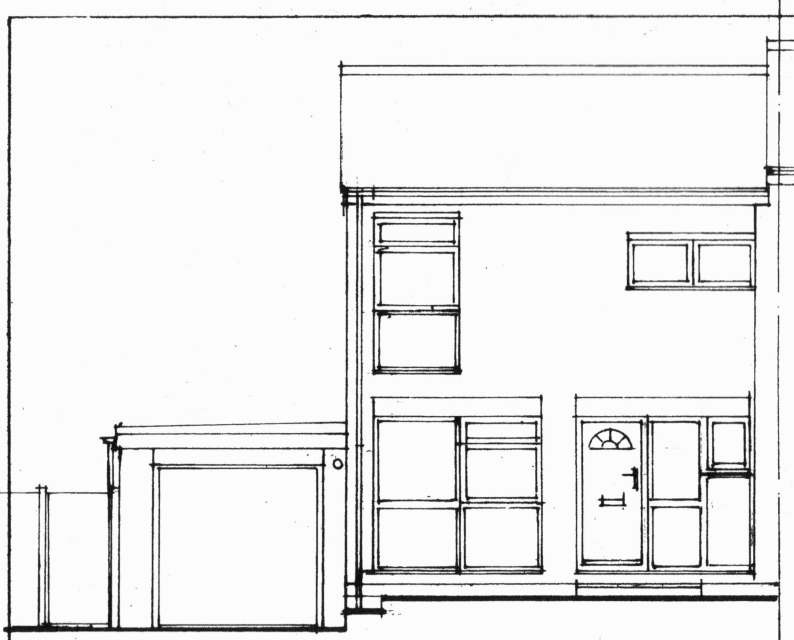
front 1:100
