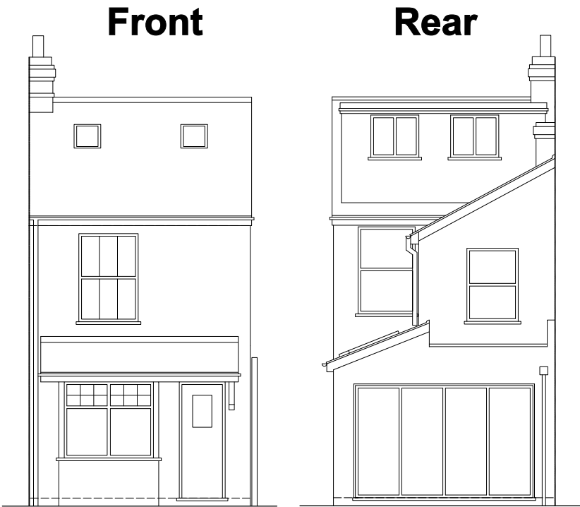
EXISTING ELEVATION
