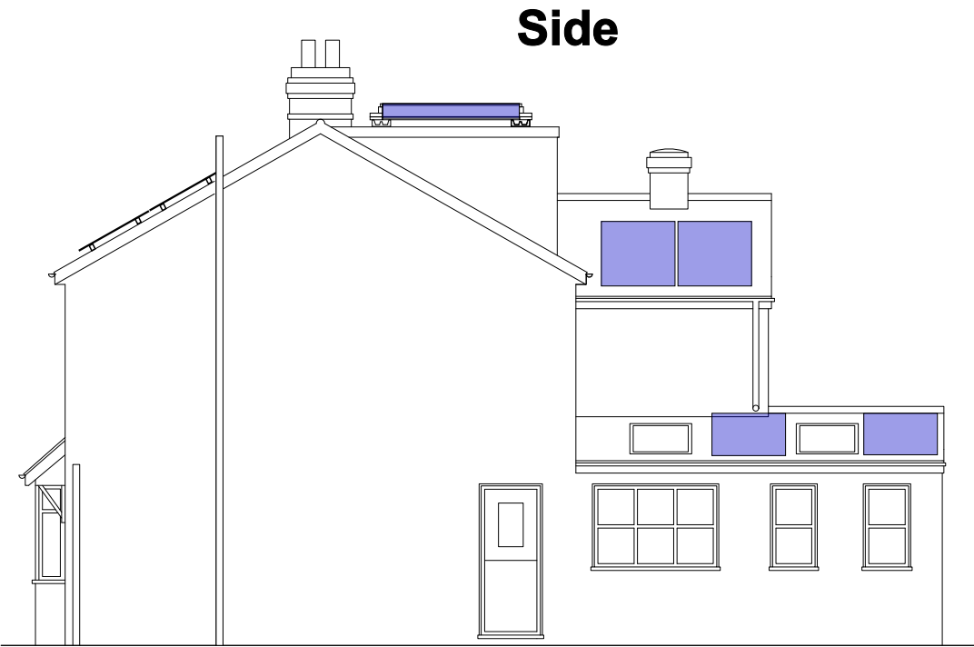
PROPOSED ELEVATION
