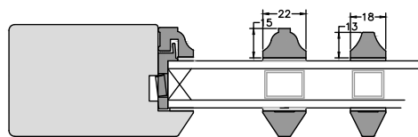
LAMBS TONGUE GLAZING BAR OPTIONS
