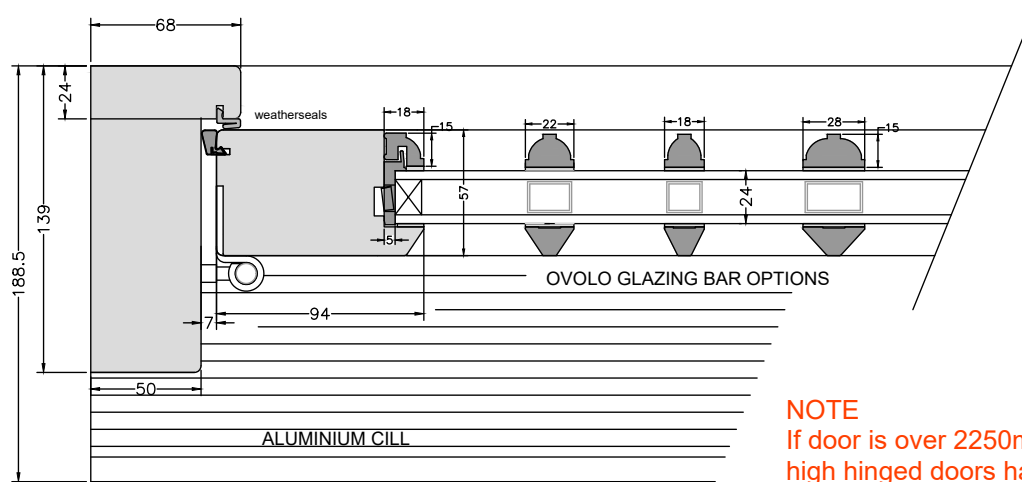
Section through Jamb
