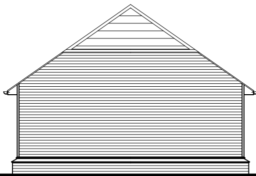
South Elevation
