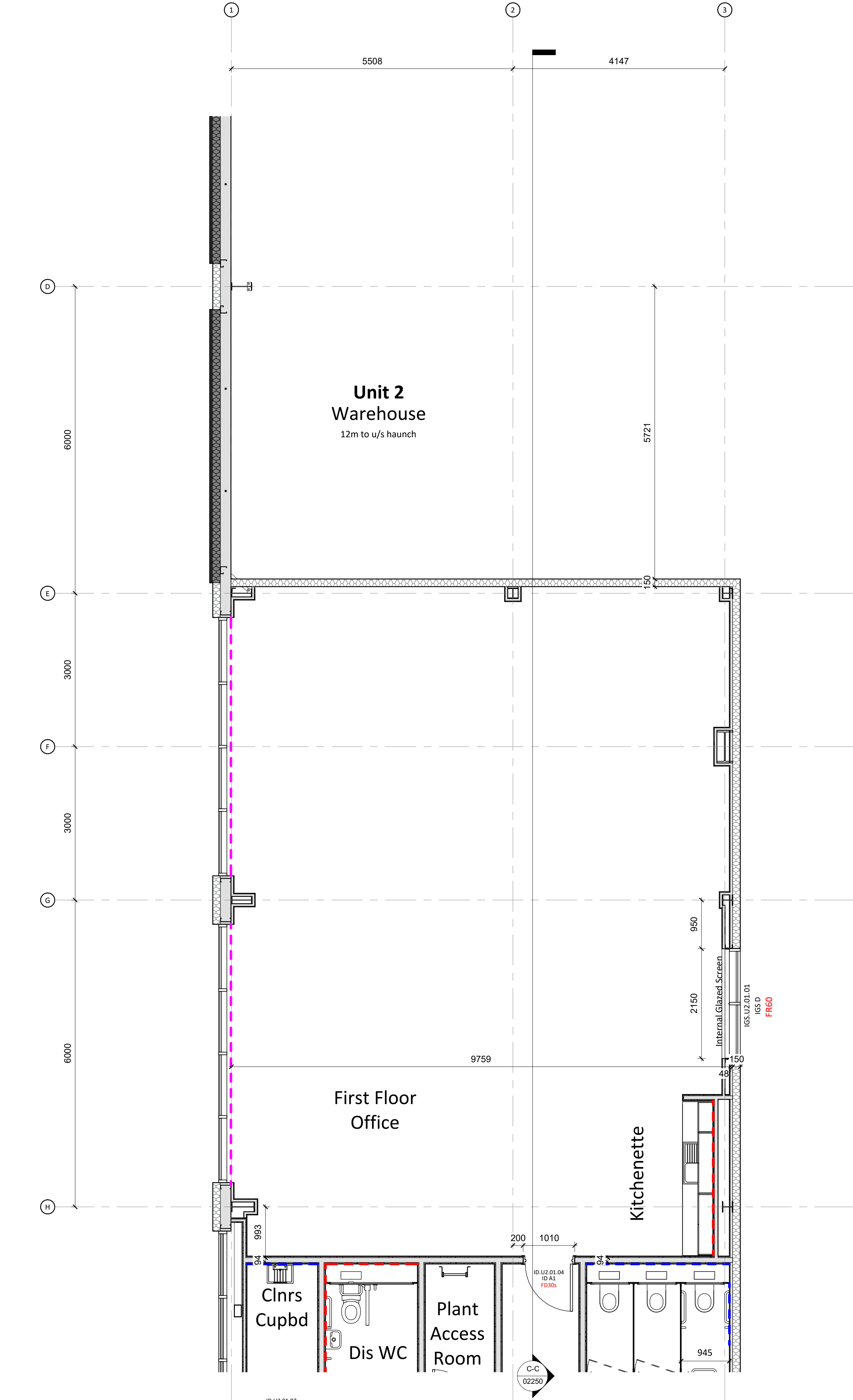
2 Unit 2 - 01 First Floor Core Plan - Part 2 1 : 50
