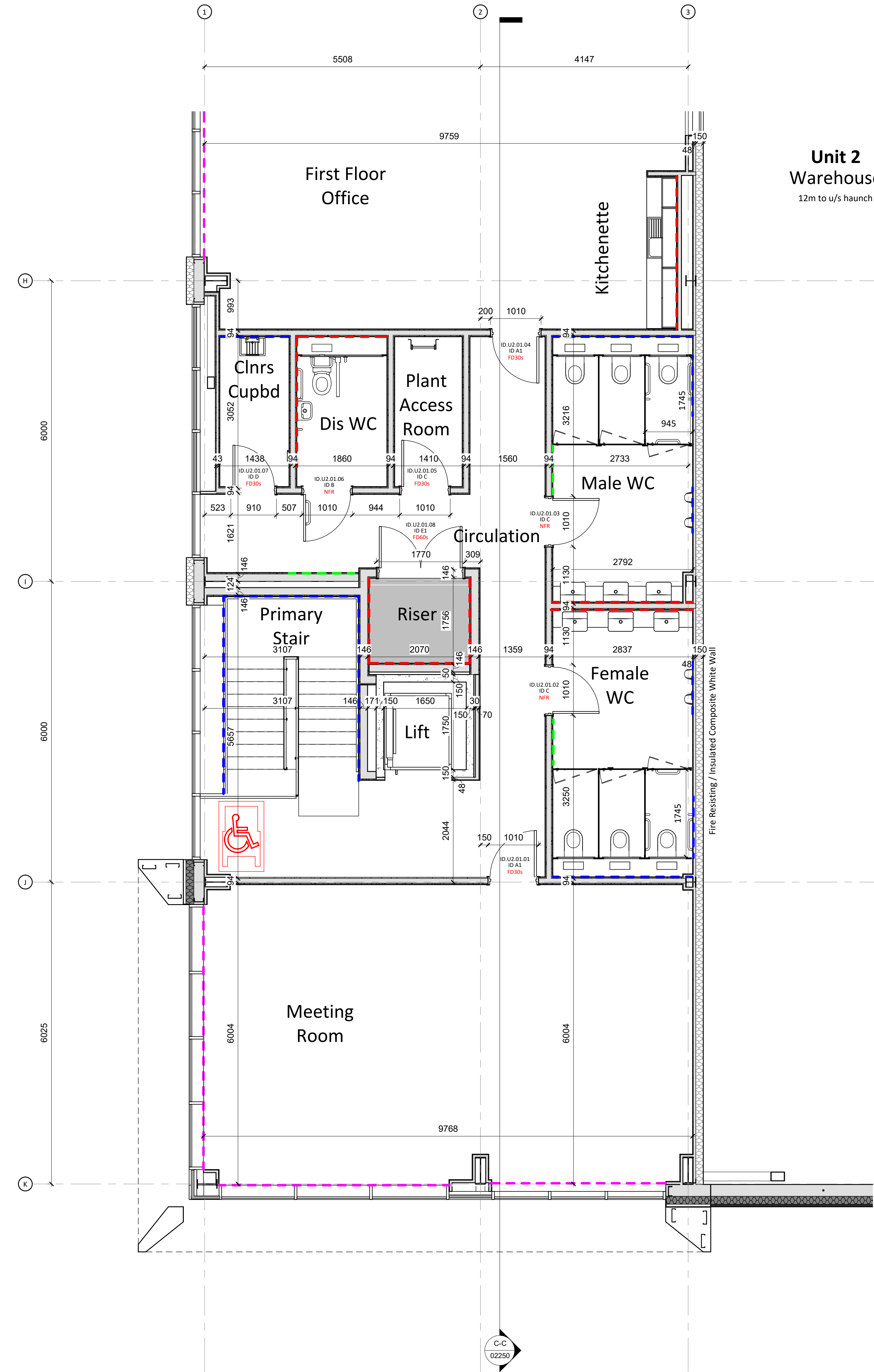
1 Unit 2 - 01 First Floor Core Plan - Part 1 1 : 50
