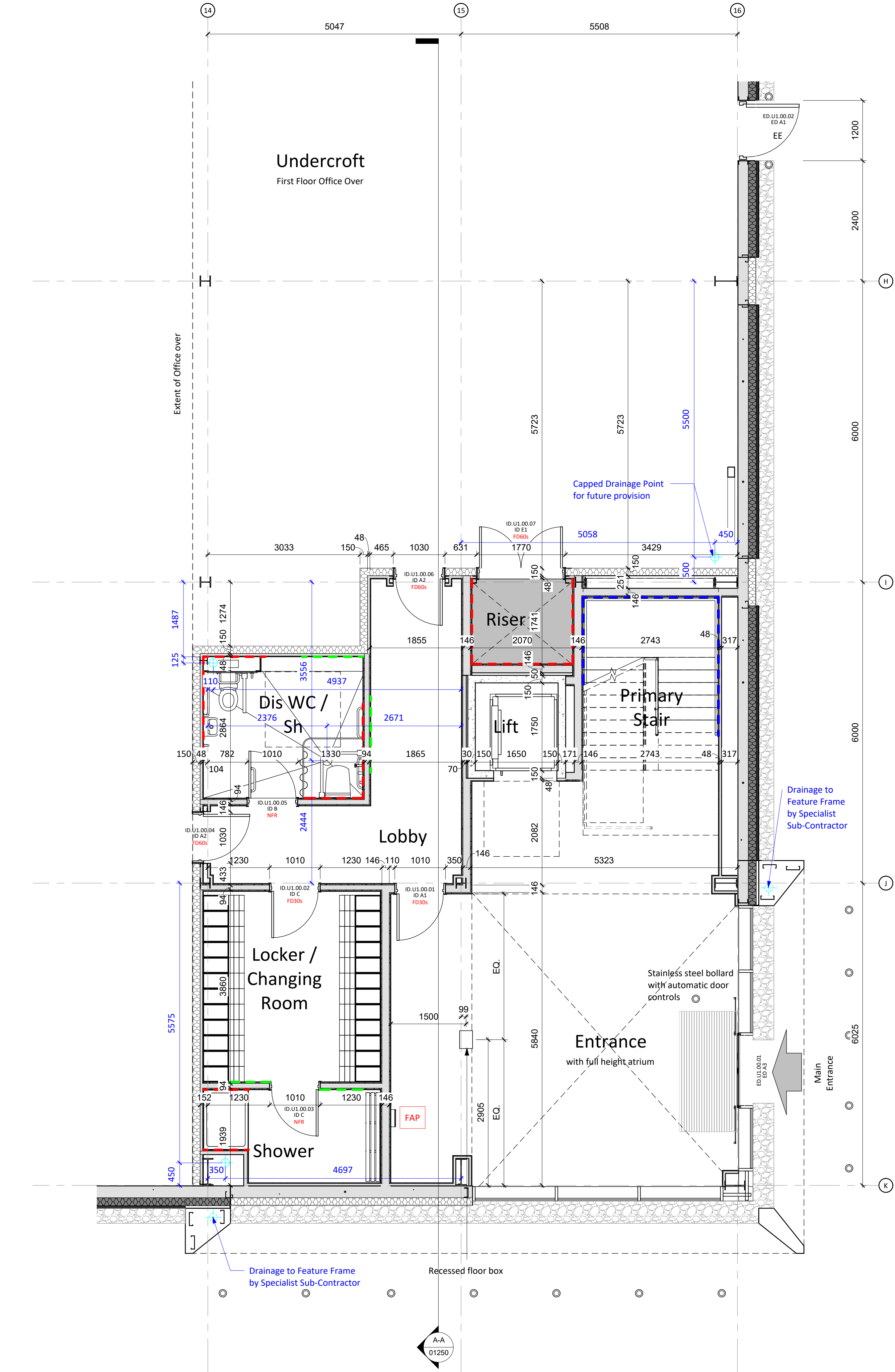
1 Unit 1 - 00 Ground Floor Core Plan - Part 1 1 : 50
