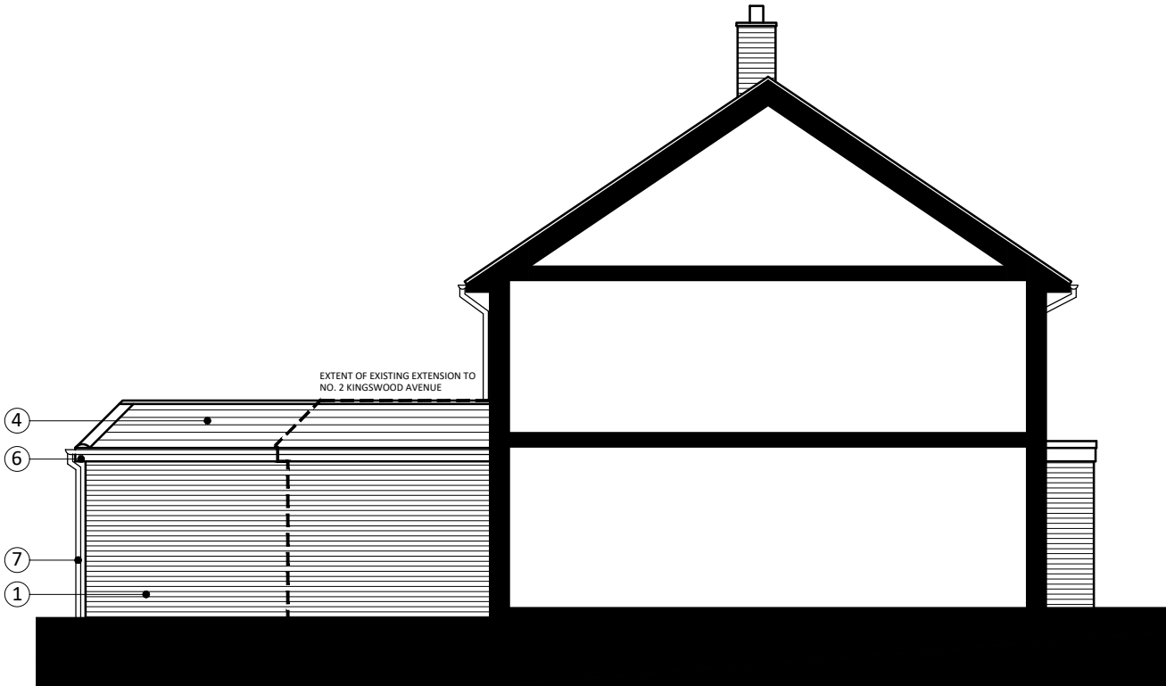
SIDE ELEVATION (B-B)
