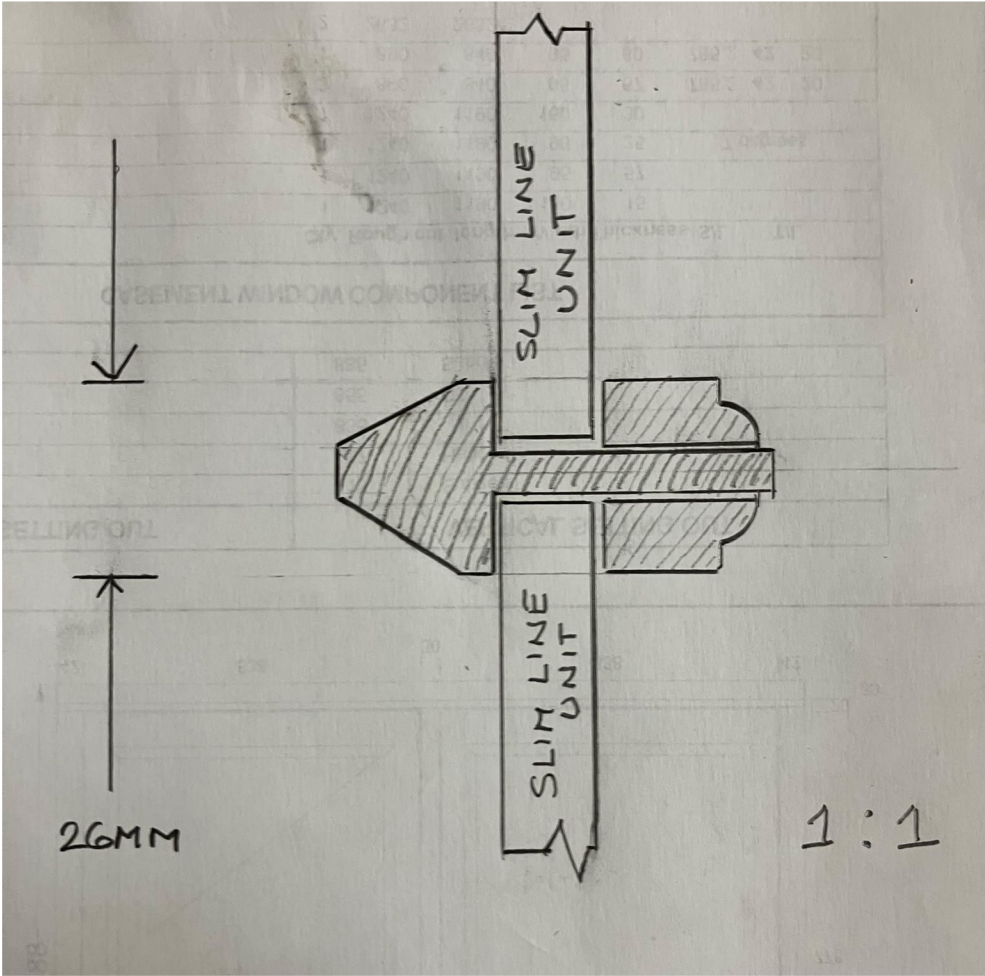
Glazing bar profile detail
