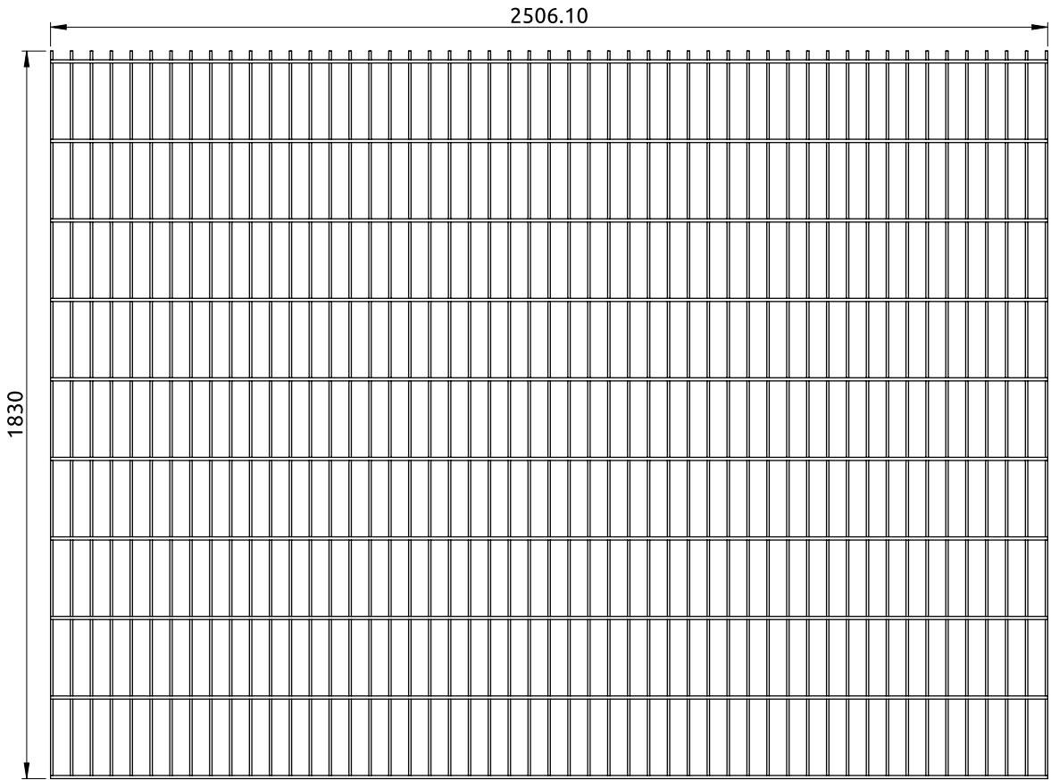
FACE VIEW
