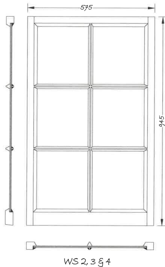
Drawing of proposed casement details
