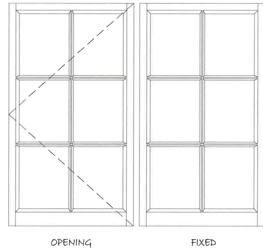
Drawing of Proposed Window Casements (within existing frame)
