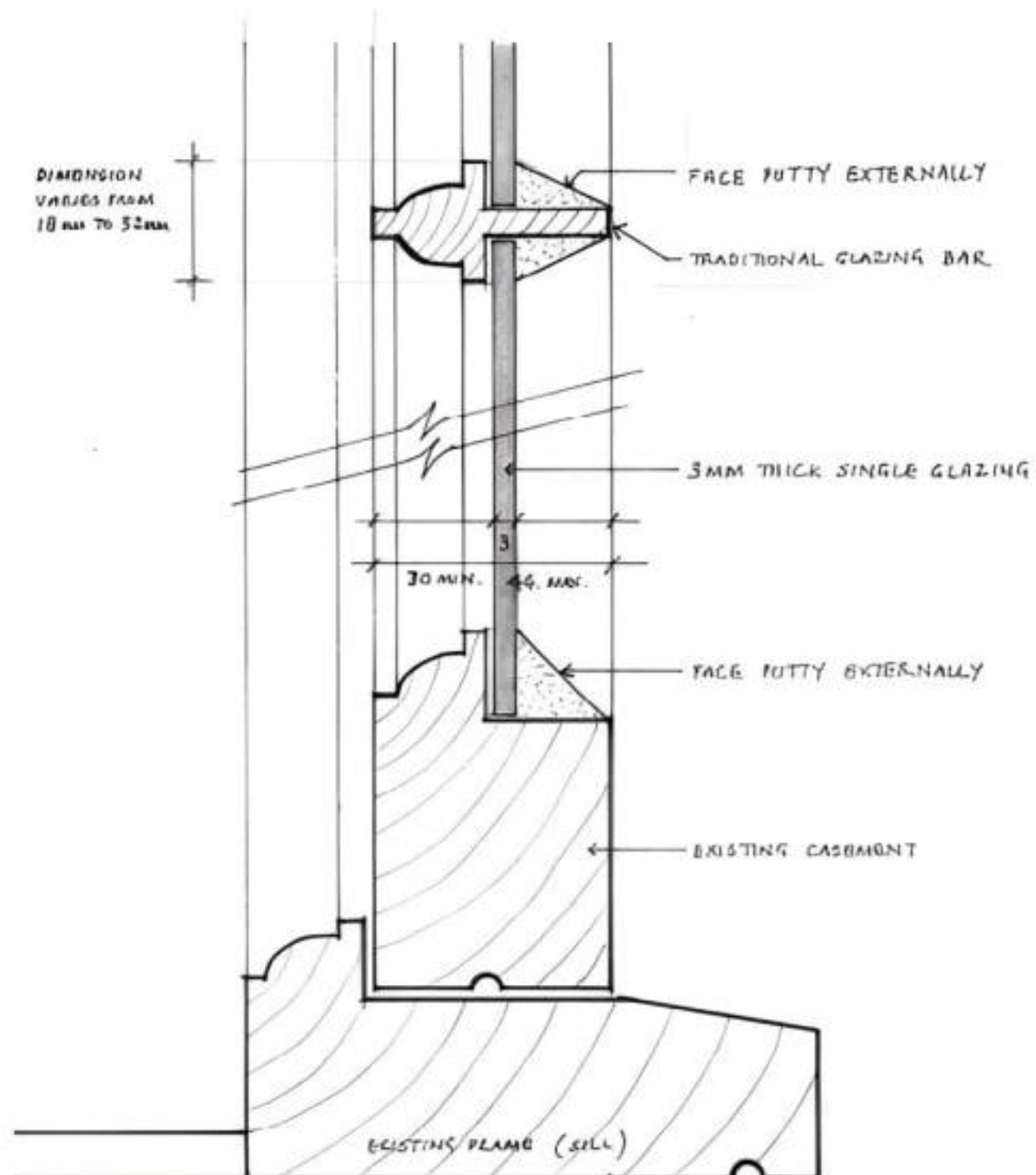
TYPICAL EXISTING WINDOW DETAIL
