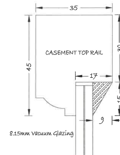
SECTION THROUGH CASEMENT TOP RAIL
