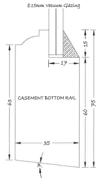
SECTION THROUGH CASEMENT BOTTOM RAIL
