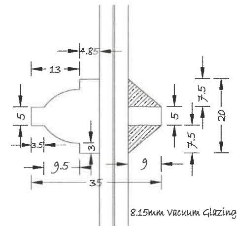
SECTION THROUGH GLAZING BARS
