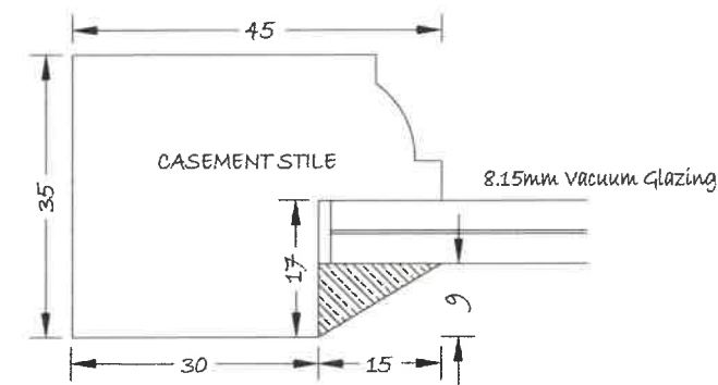
SECTION THROUGH CASEMENT STILE
