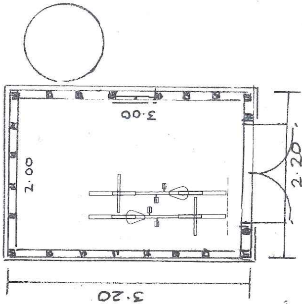
FLOOR PLAN
