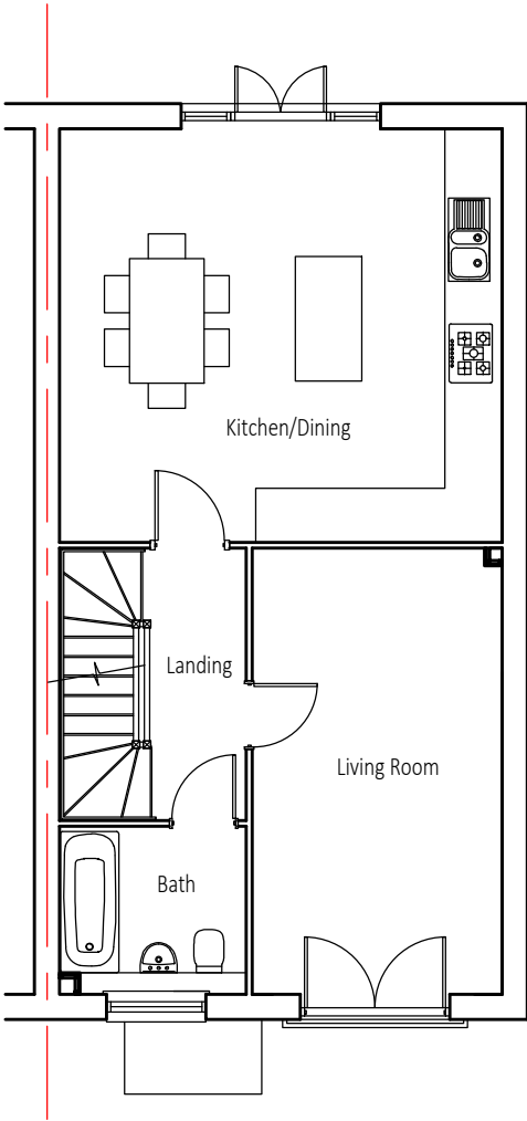
First Floor Plan (unchanged) @ 1/100
