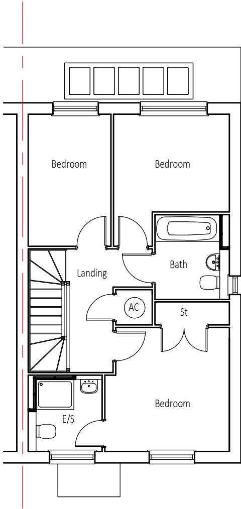
Second Floor Plan (unchanged) @ 1/100
