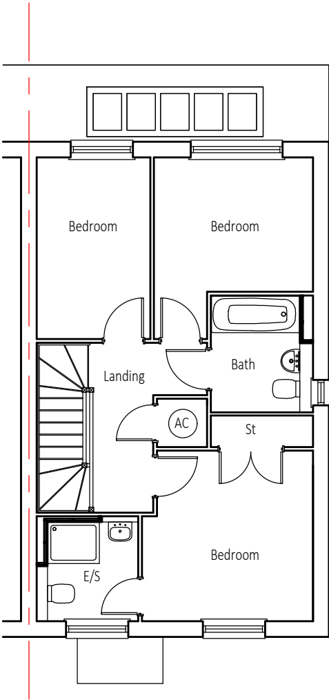
Second Floor Plan @ 1/100
