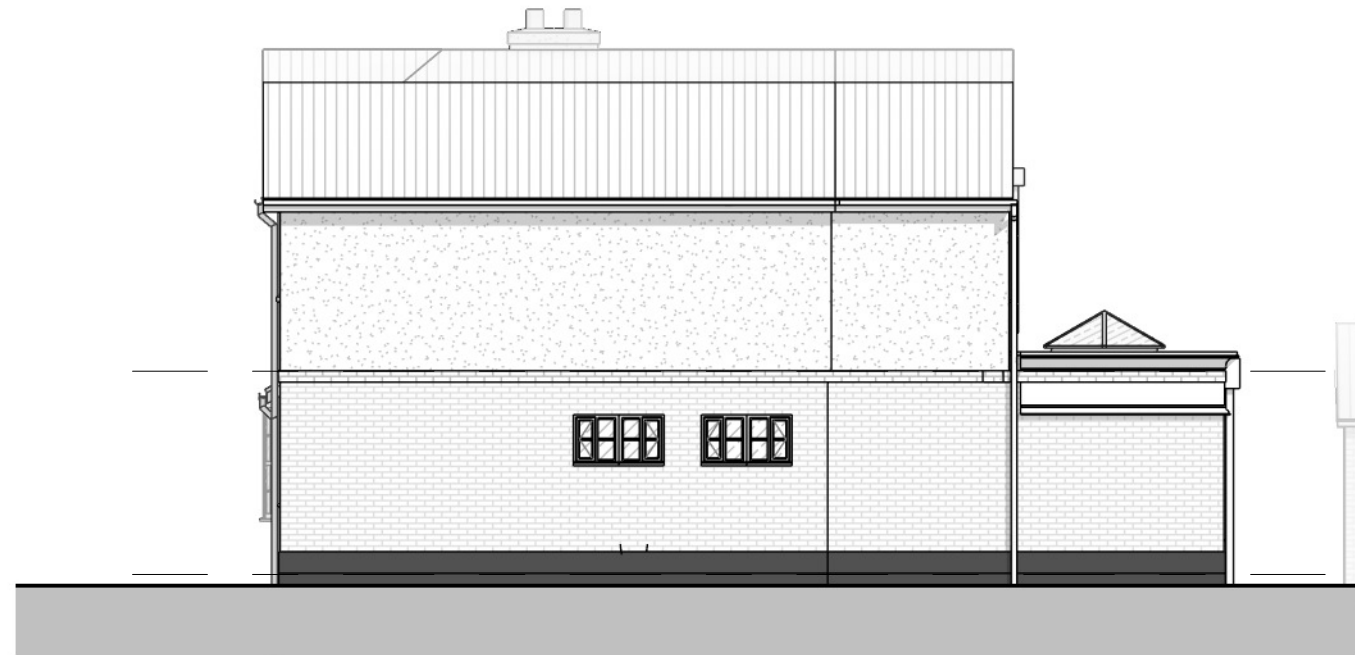
2 Party Wall Elevation - PROPOSED - B 1 : 100 @A3
