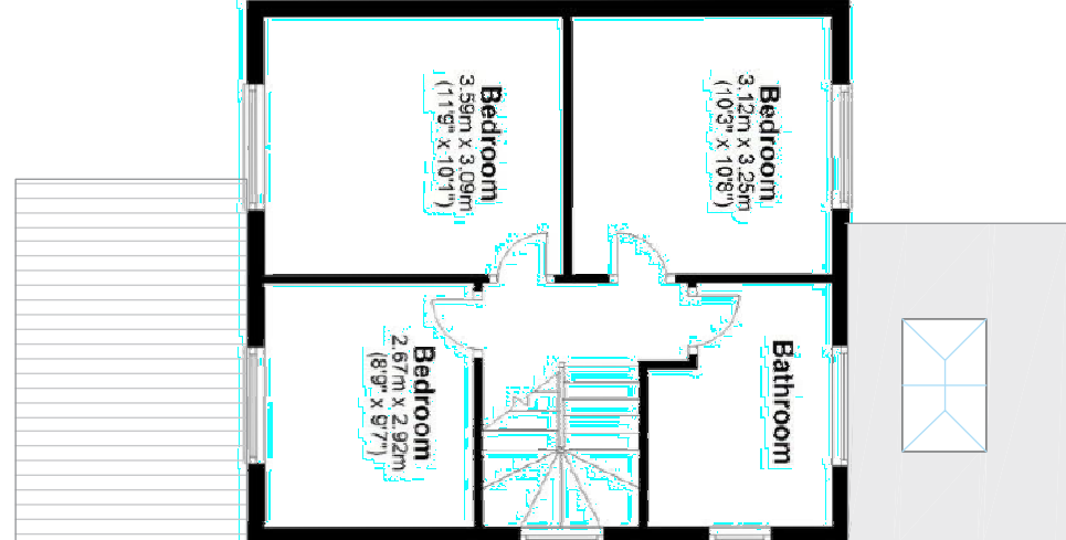
Existing First Floor Plan /Roof plan. (1:100 scale)
