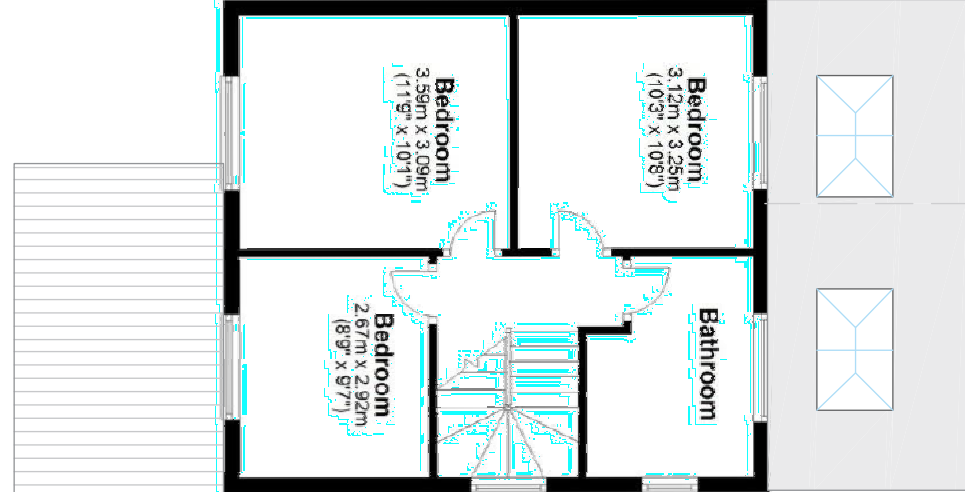
Proposed First Floor Plan /Roof plan. (1:100 scale)
