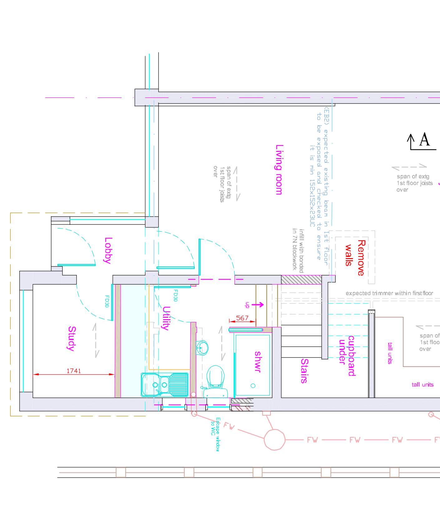
Proposed Ground Floor Plan. (1:50 scale)
