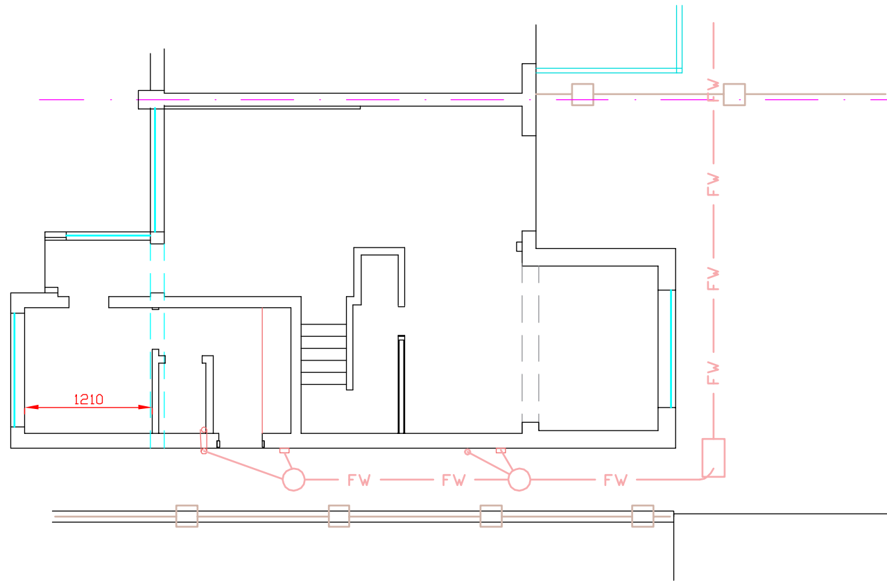
Existing Ground Floor Plan. (1:100 scale)
