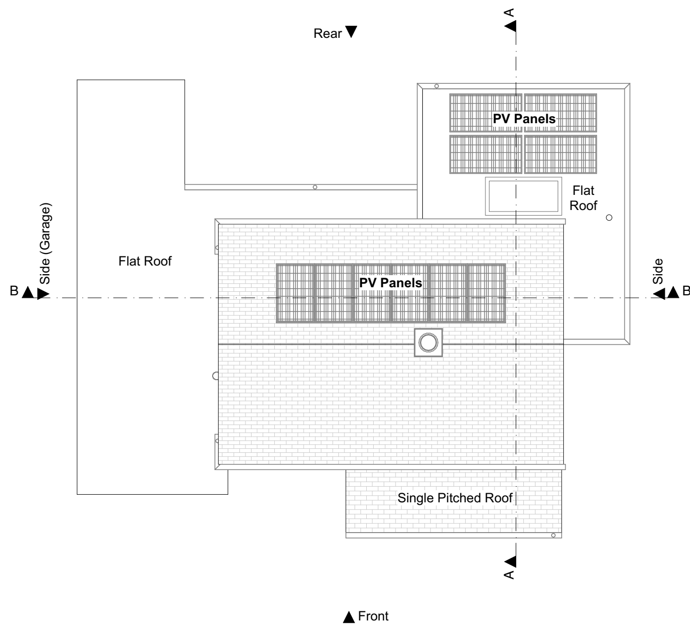
2. Roof PLANNING 1:100
