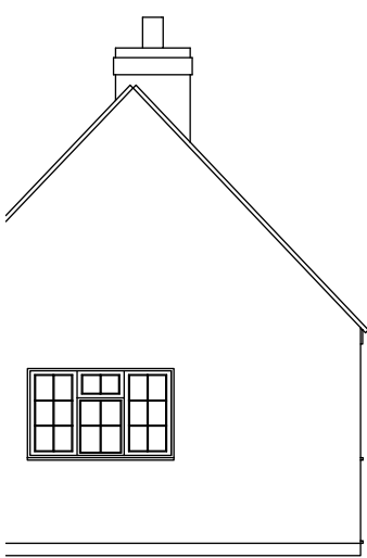
West Elevation Proposed
