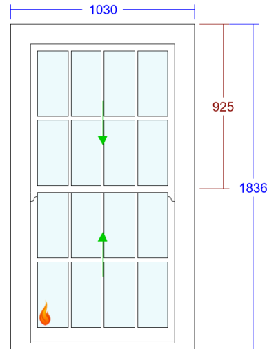
5. Slim Sash Window (Playroom)
