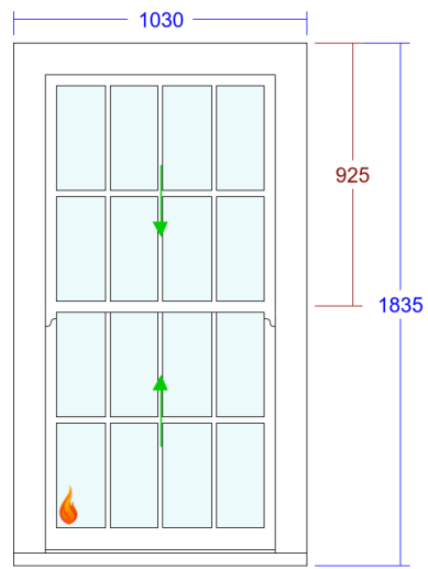
7. Slim Sash Window (Office)
