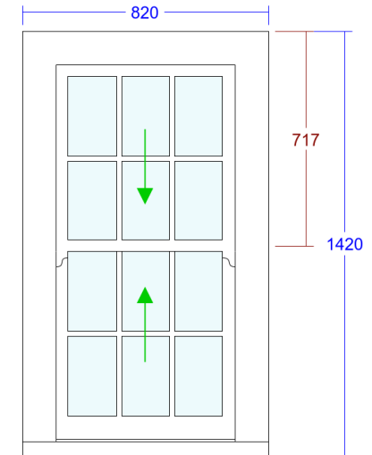
3. Slim Sash Window (Living Room Side)
