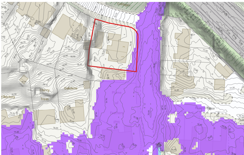
Figure 3. Flood Inundation Map (1 in 75 year)
