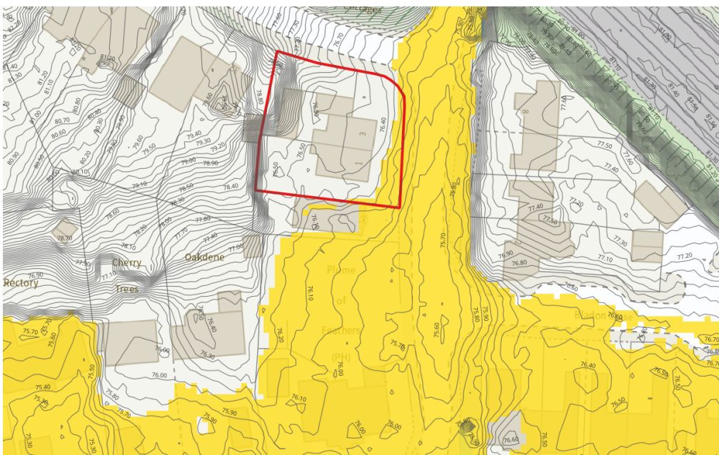
Figure 6. Flood Inundation Map (1 in 100 year + 30% CC)
