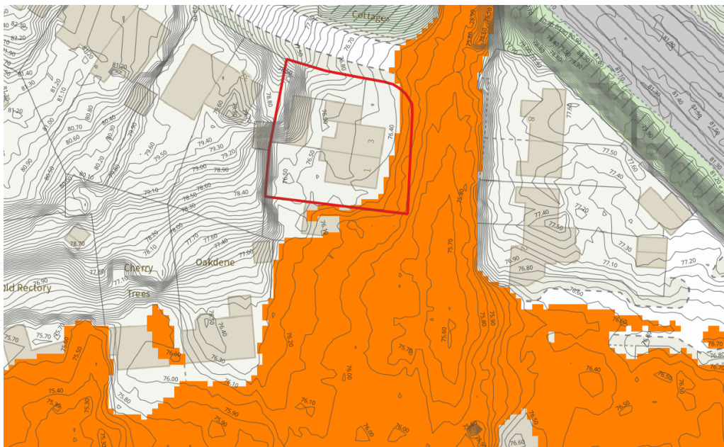
Figure 10. Flood Inundation Map with culvert completely blocked (1 in 1000 year + 19% CC)
