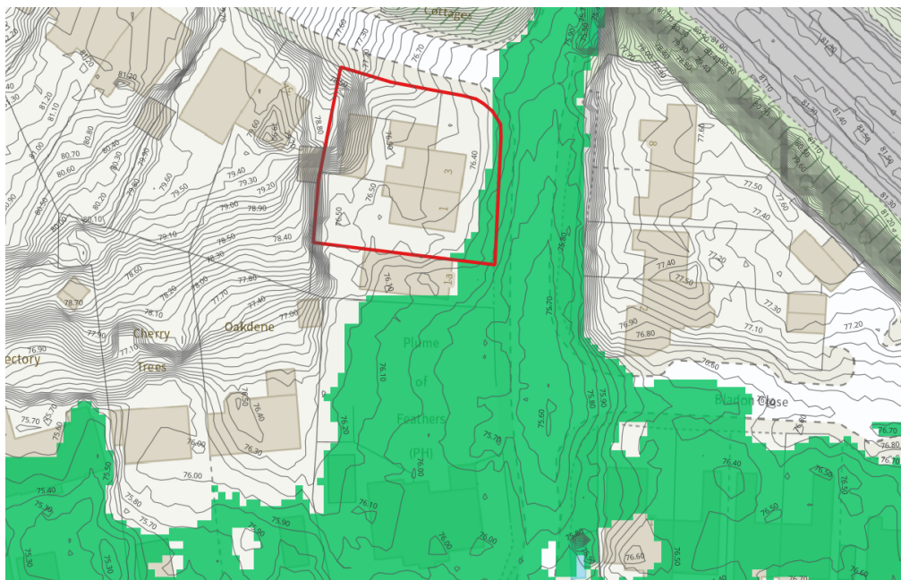
Figure 4. Flood Inundation Map (1 in 100 year)
