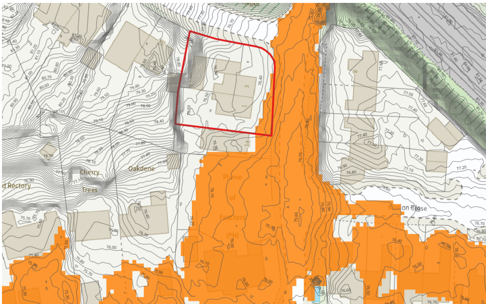
Figure 2. Flood Inundation Map (1 in 30 year)
