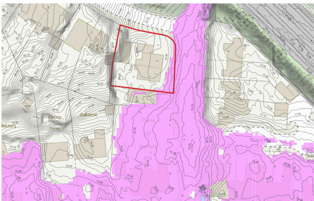
Figure 5. Flood Inundation Map (1 in 100 year + 19% CC)
