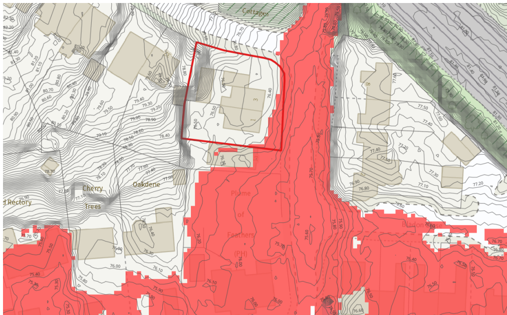
Figure 7. Flood Inundation Map (1 in 200 year)
