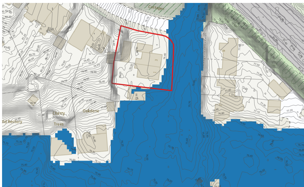
Figure 9. Flood Inundation Map (1 in 1000 year + 19% CC)
