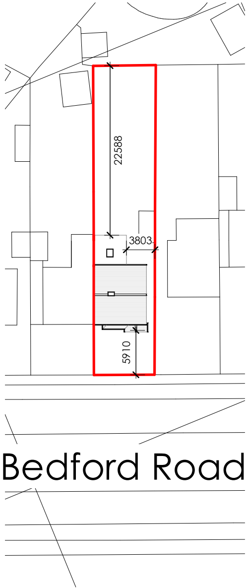
1 Proposed Roof Plan 1 : 500
