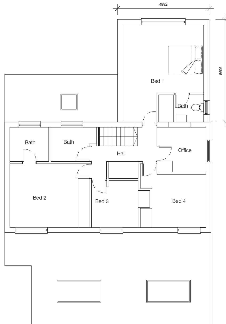
Proposed First Plan 1:100
