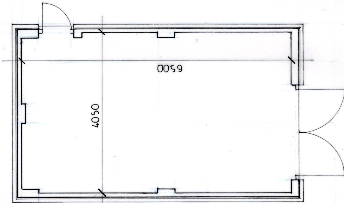
Floor Plan
