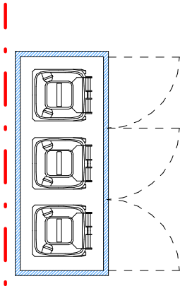
Proposed Plan - Bin Store 1 : 50
