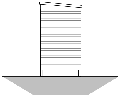
Proposed Side B Elevation - Bin Store 1 : 50
